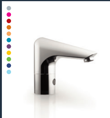
Sensorflow 21 Electronic one taphole basin spout, suitable for pre-mixed water. Anti-vandal and water economy properties make this outlet suitable for every building. Laminar flow internal design ensures water-borne bacteria are minimised. The sensor also shuts off water supply if obstructed ( above, top ). A4171AA Mains Transformer A4172AA Links Box A4122AA Battery
