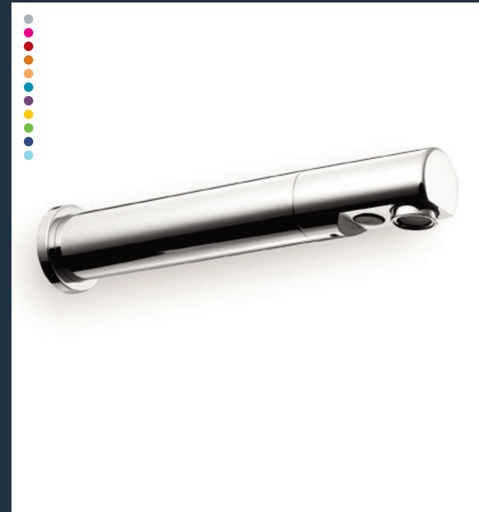
Sensorflow 21 Compact Compact 230mm basin wall spout with built in sensor, suitable for pre-mixed water (above) . A4849AA Mains Transformer A4850AA Links Box A4848AA Battery
