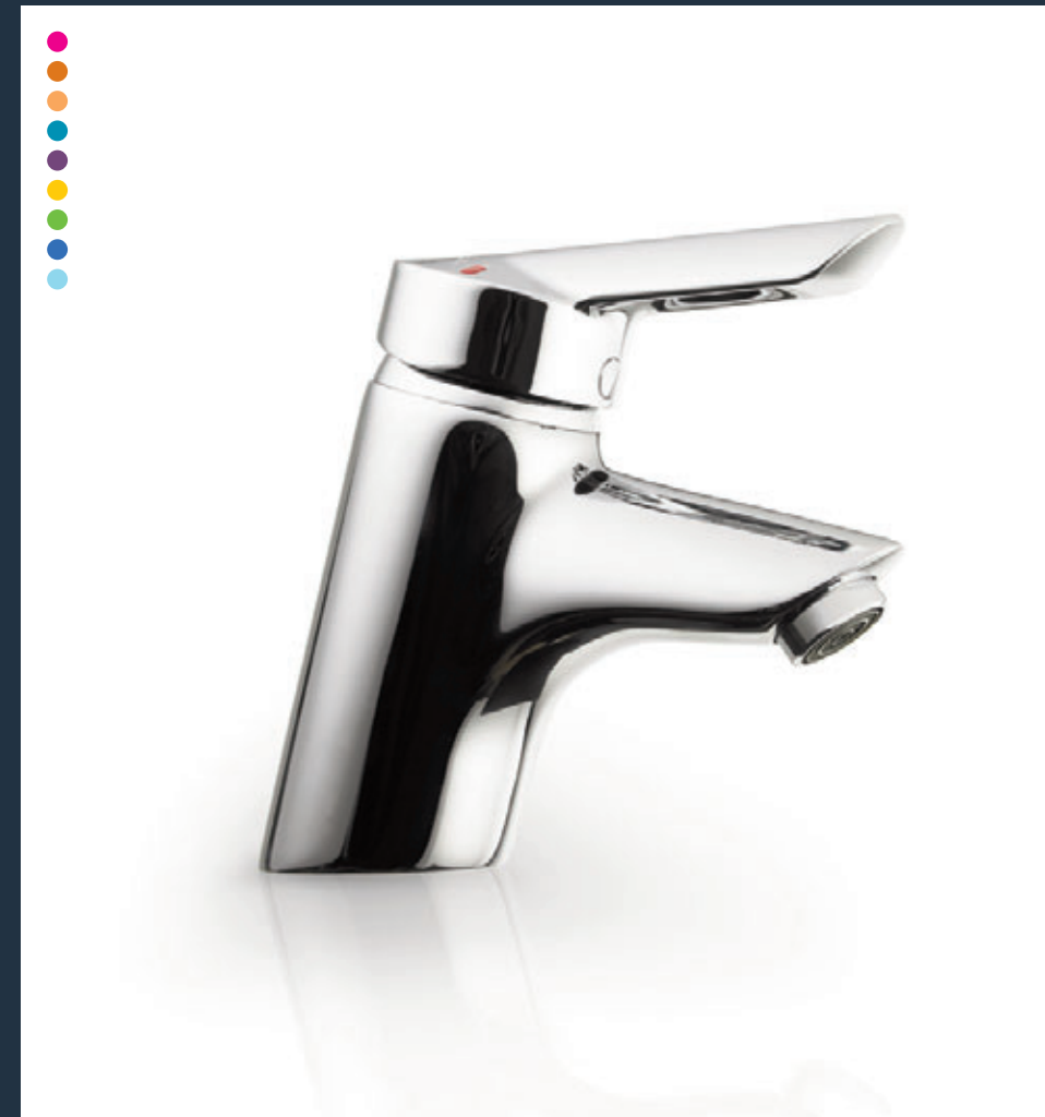
B8260AA Piccolo 21 Single lever monoblock basin mixer, without pop-up waste. This tough and easy to clean design has clear hot/cold identification that will not wear off and a special seal to protect the ceramic disc cartridge from harsh cleaning fluids. Water economy is optimised by CLICK technology. SPX hoses, built in temperature stop and laminar flow design make this a safe and hygienic mixer (above).
