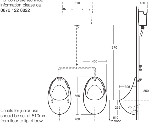
S611001 Contour urinal (above) .
