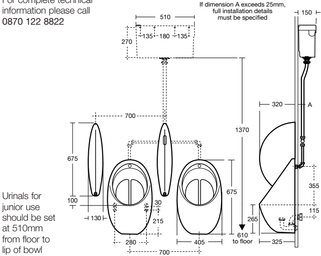
S611901 Contour hygienIQ urinal (above) .
