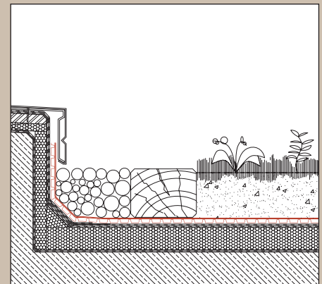
Herbaceous roof detail – fascia with metal cover.
