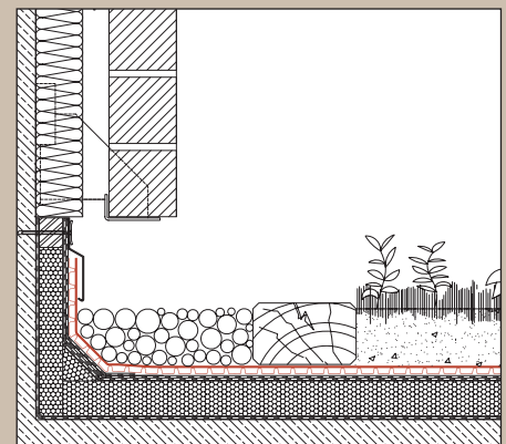
Herbaceous roof detail – connection to a double-shelled masonry structure.
