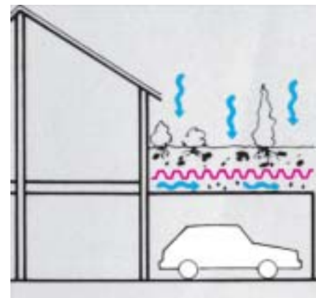
Installed under roof terraces and parking lots, DELTA®-TERRAXX and DELTA®-NP DRAIN make sure that any precipitation is drained away safely.
