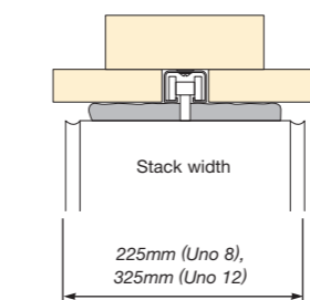
Track with acoustic seal
