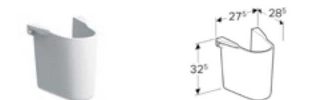
Geberit Selnova semi pedestal W 27.5 / D 28.5 / H 32.5cm For use with 65/55/50cm washbasins.
