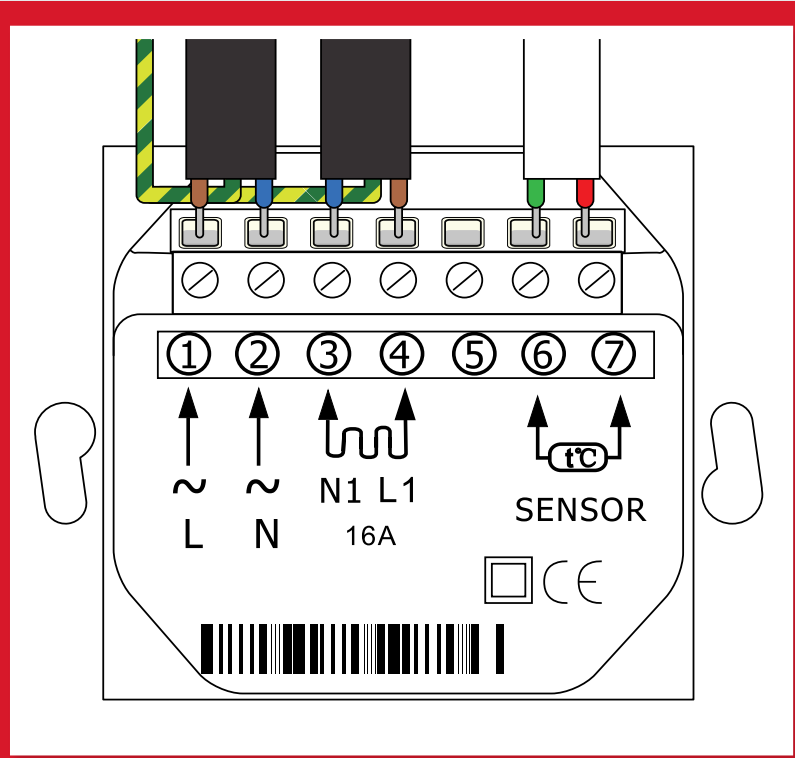
Simple wiring diagram
