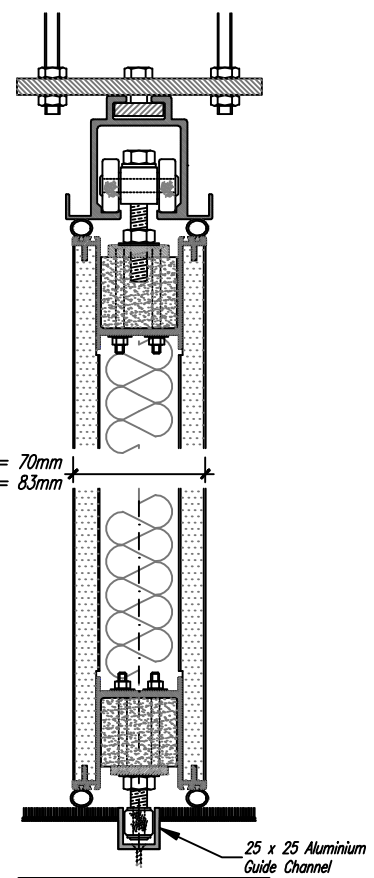
TOP HUNG
