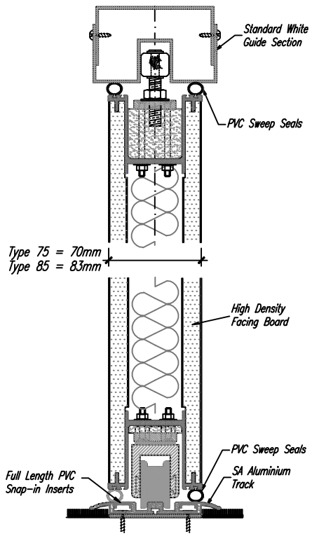
BOTTOM RUNNING
