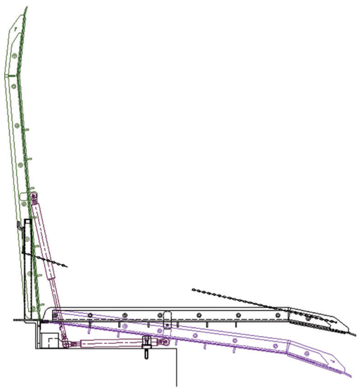
Droprite Platform Unit Side View Movement illustrations
