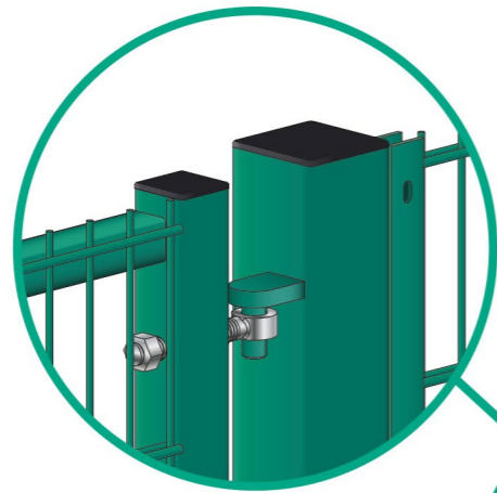
Hinge Detail
