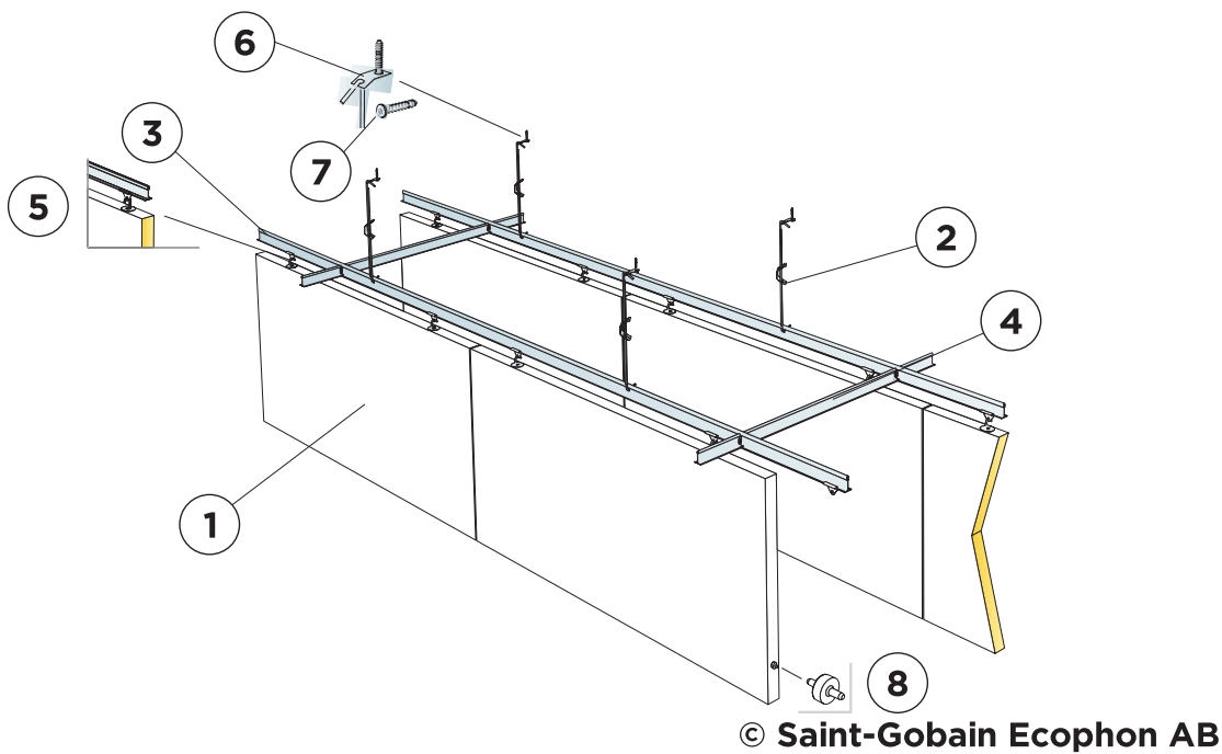
Installation diagram (M494C4) for Ecophon Hygiene Performance™ Baffle C4 (in rows)
