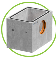
BG-DELTA T sand trap element 460mm x 960mm height with 315Ø outlet
