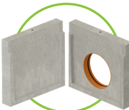
Example of groove end cap, with and without outlet
