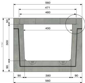
Cross section of BG-DELTA U 400mm x 300mm channel with 50mm edge height
