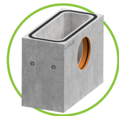
BG-DELTA U Type-1 460mm x 960mm sand trap element with 315Ø outlet
