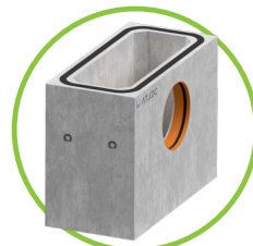
BG-DELTA T Type-1 460mm x 960mm sand trap element with 315Ø outlet
