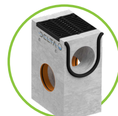
BG-DELTA O sand trap element with 2 side connections and removable top grating
