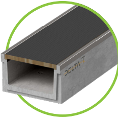
Channel with 25mm galvanised edge height - shown with B 125 wooden cover
