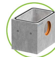
BG-DELTA U Type-2 660mm x 960mm sand trap element with 315Ø outlet
