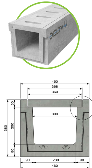
Cross section of BG-DELTA U 300mm x 250mm channel with 50mm edge height
