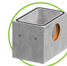
BG-DELTA U Type-2 660mm x 960mm sand trap element with 315Ø outlet
