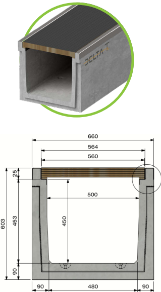
BG-DELTA T 500mm x 450mm with 25mm galvanised edge height cross section - shown with wooden cover
