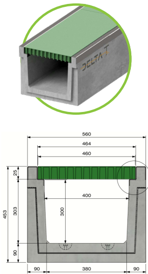
BG-DELTA T 400mm x 300mm with 25mm galvanised edge height cross section - shown with plastic cover
