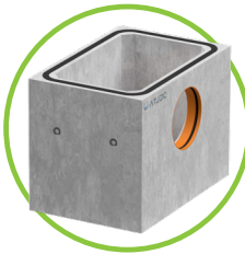
BG-DELTA T Type-2 660mm x 960mm sand trap element with 315Ø outlet
