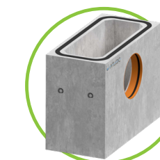
BG-DELTA U Type-1 460mm x 960mm sand trap element with 315Ø outlet
