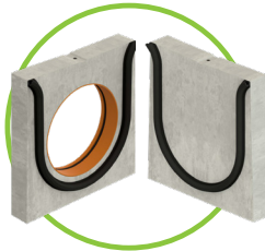
BG-DELTA O end caps with rubber seal
