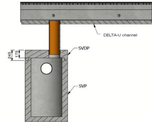
Sludge trap cover with 400mm diameter opening for PVC pipe connection
