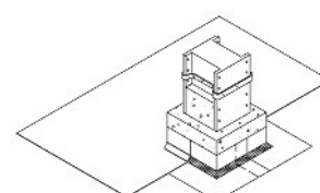
ColumnStop End SF/BB
