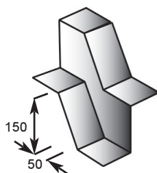
Change of Level BB
