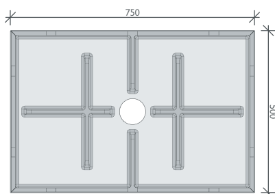
step 750/500/80 (smaller and larger alternative available)
