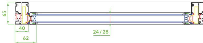
Plan view double element
