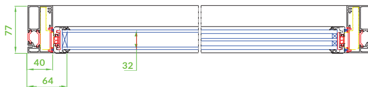
FLW 32_0 double glazing
