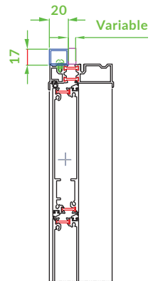
Adapter type A 17/20
