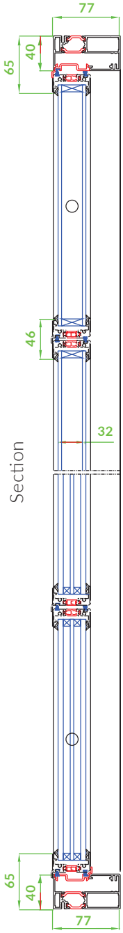
FLW 32_0 triple glazing
