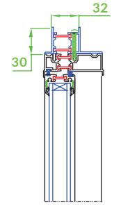
Adapter type B 30/32
