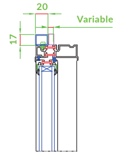
Adapter type A 17/20
