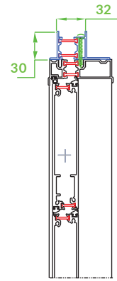
Adapter type B 30/32
