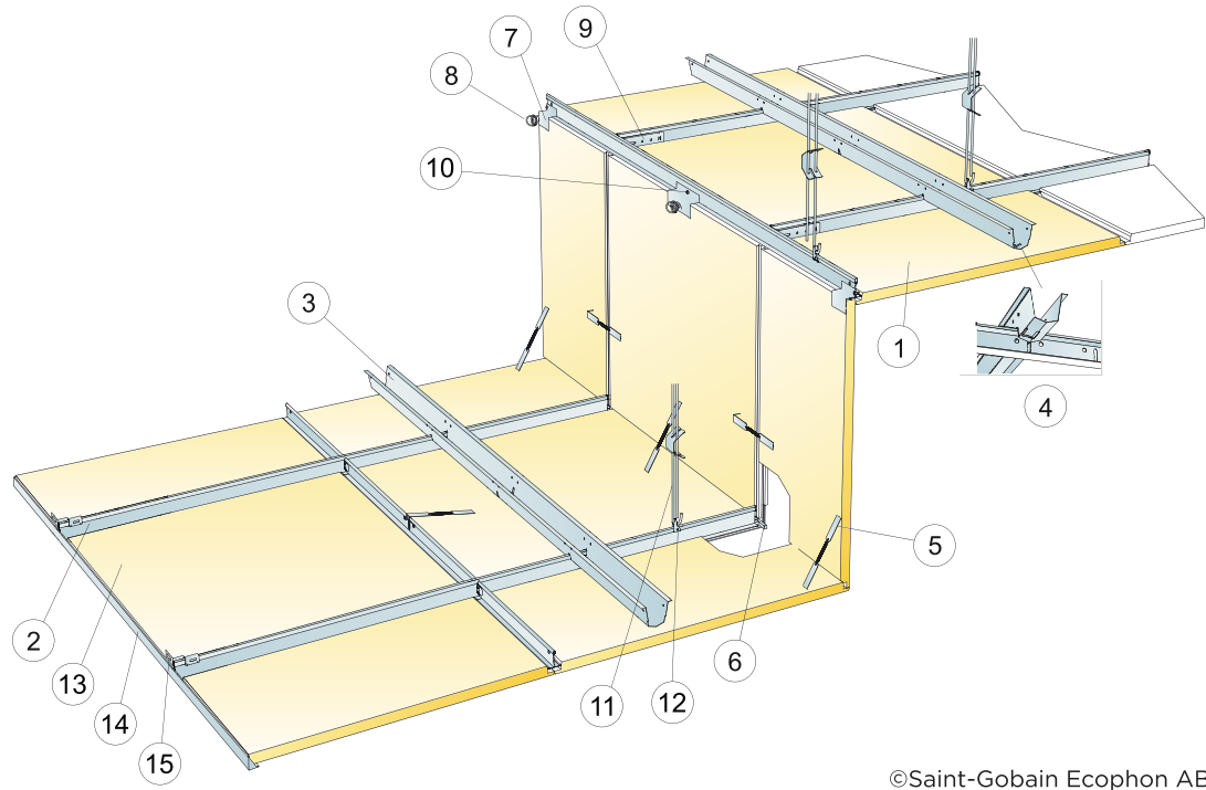
©Saint-Gobain Ecophon AB Installation diagram (M613) for Ecophon Focus Ds Level change. Suspended installation
