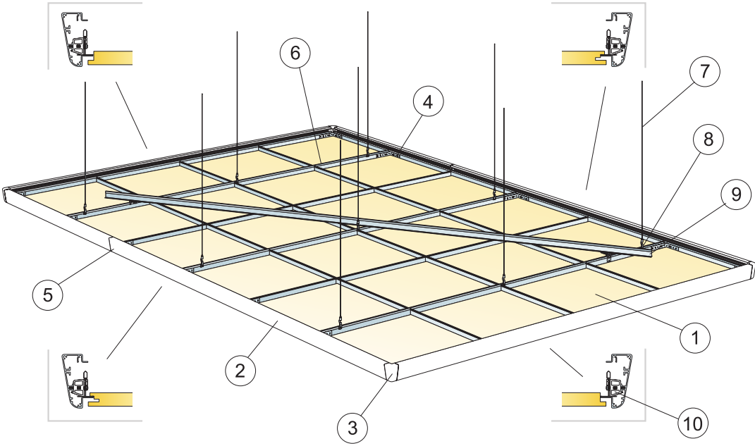
© Saint-Gobain Ecophon AB Installation diagram (M211) for Ecophon Edge 500 with Focus Dg
