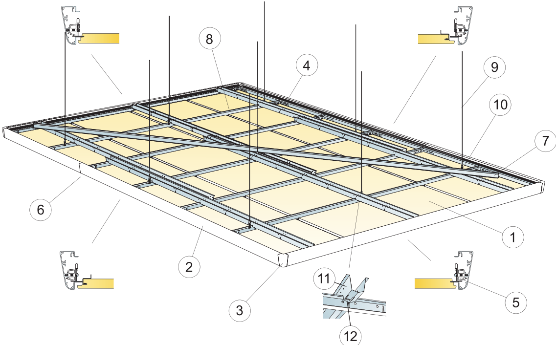
Installation diagram (M210) for Ecophon Edge 500 with Focus Ds
