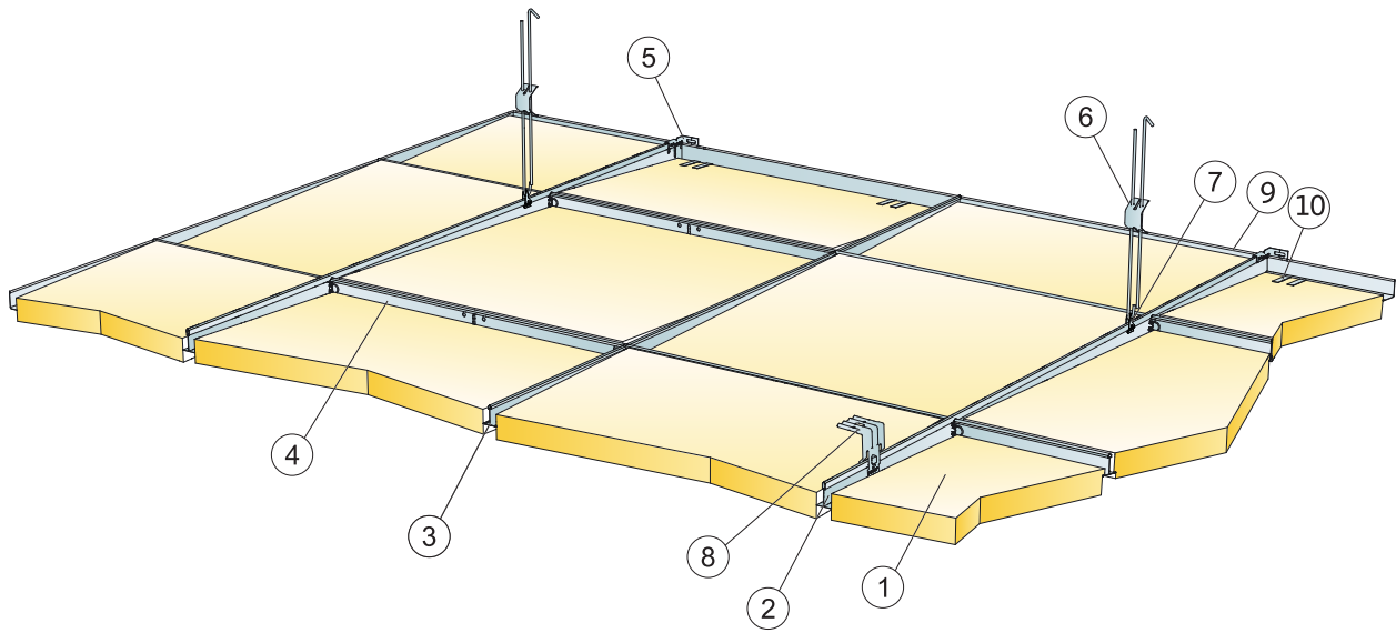
Installation diagram (M393) for Ecophon Focus Ez
