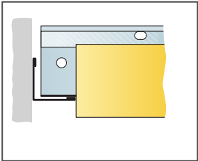
Wall connection non-supported edge
