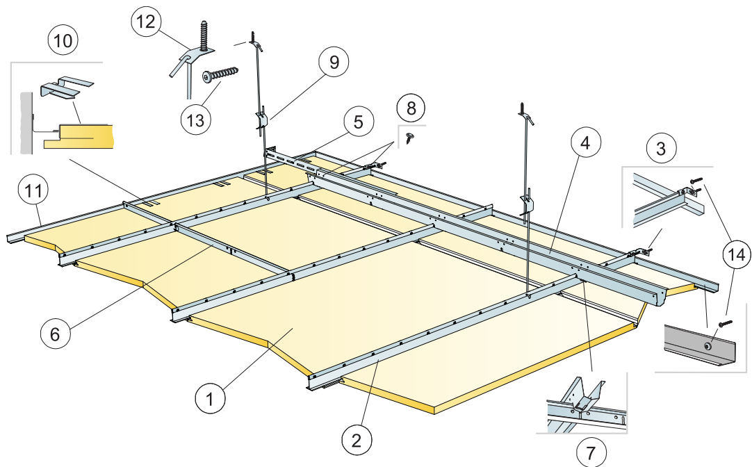
Installation diagram (M676C4) for Ecophon Hygiene™ Black Ds C4. Suspended installation
