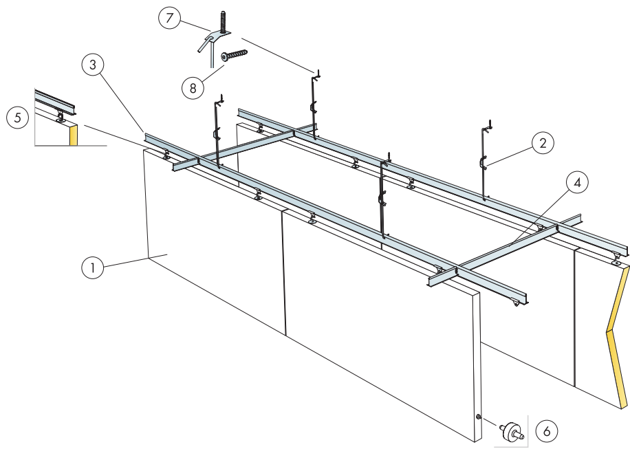
© Saint-Gobain Ecophon AB Installation diagram (M494C4) for Ecophon Hygiene Performance™ Baffle C4 (in rows)
