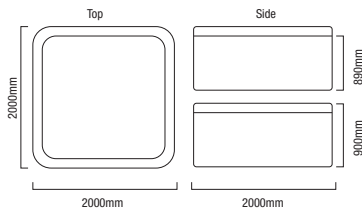
Structure Frame drawing of BREVA
