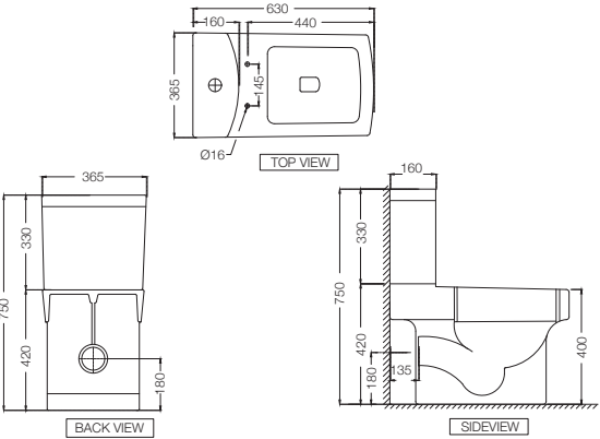
FNS-WHT-40751P180UFSMZ Bowl With Cistern For Coupled WC With UF Soft Close Slim Seat Cover, Hinges, Dual Flush Cistern Fitting And Fixing Accessories, Size: 365x630x750 mm, P Trap-180 mm £ 344
