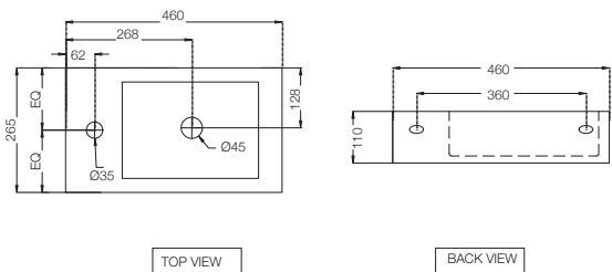
JDS-WHT-25801 Counter Top Basin, Size: 460x265x110 mm £ 84
