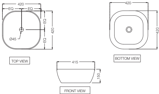
JDS-WHM-25911 Thin Rim Counter Top Basin In White Matt, Size: 420x420x150 mm, Shape - Square £ 126
