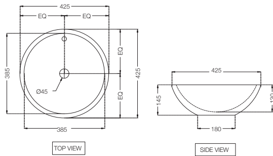
ONS-WHT-10901 Counter Top Basin, Size: 425x425x145 mm £ 107
