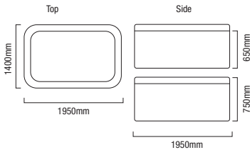
Structure Frame drawing of NUOVO
