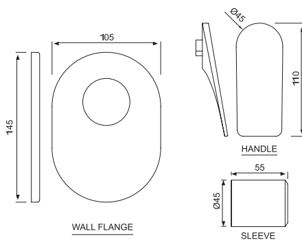
Manual Single outlet Mixer Trim Kit (Compatible In-wall Parts ALD-227 or ALD-229 are sold separately)
