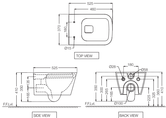
LAS-WHT-91953BIUFMS Rimless Blind Installation Wall Hung WC With UF Soft Close Slim Seat Cover, Hinges, Accessories Set, Size: 370x525x350 mm £ 434
