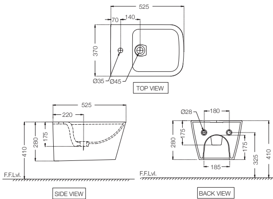
LAS-WHT-91153 Blind Installation Wall Hung Bidet With Fixing Accessories, Size: 370x525x280 mm, £ 236
