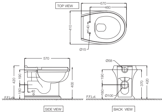
QPS-WHT-7955P180UFPM Rimless Back To Wall WC - Floor Mounted With UF Soft Close Seat Cover, Hinges, Fixing Accessories And Accessories Set, Size: 410x570x420 mm, P Trap- 180 mm £ 381
