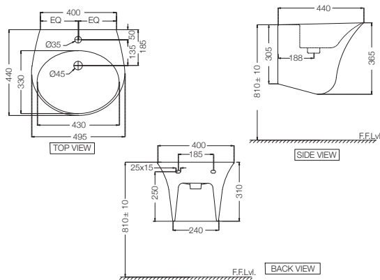
ONS-WHT-10801 Wall Hung Integrated Basin With Fixing Accessories, Size: 495x440x365 mm £ 230
