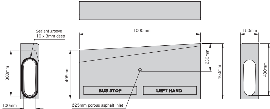
HB405 left-hand bus stop transition kerb
