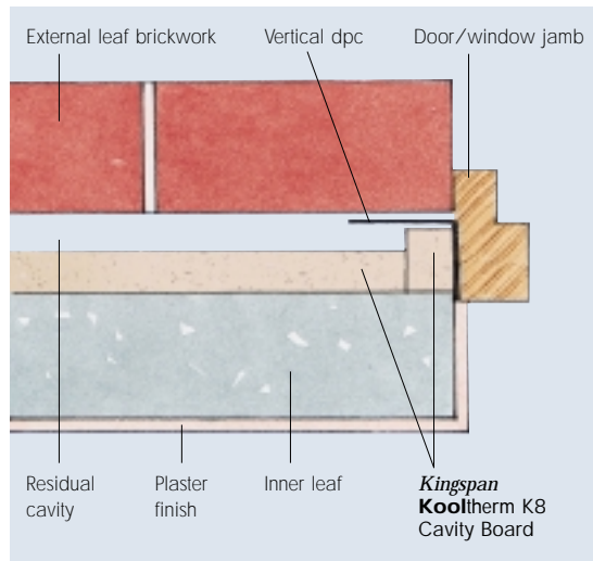
Figure 3 TYPICAL JAMB DETAIL
