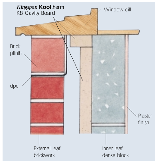
Figure 4 TYPICAL CILL DETAIL
