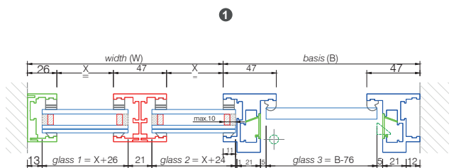
Horizontal section Basis XL/Frame XL
