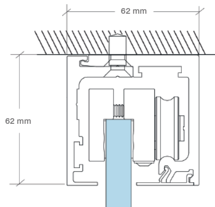
Single slider kits (Ceiling mount illustrated)
