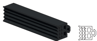
Double Glazed Fixed Profile Gasket for 20, 22 and 24mm Glass • EPDM rubber
