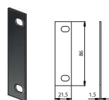
Double Glazed Support Plate for Dormer Hinge Cat. No. FXCU • For 10 to 12mm glass
