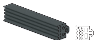
Roll-In Fixing Gasket for 8 to 16mm Glass • EPDM rubber
