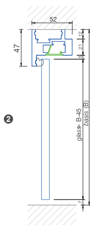
Vertical section Basis XL/ Frame XL
