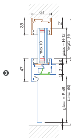
Vertical section Basis XL/ Frame XL
