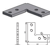
Double Glazed 90° Connector for Floor and Ceiling Profiles Cat. No. FXCH
