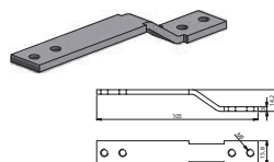
Double Glazed Z Connector Cat. No. FXCZ
