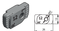
Double Glazed Hammer Head Nut Cat. No. FXHHN • For 10 to 12mm glass
