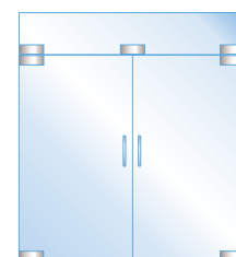
Paired doors and transom with floor closers
