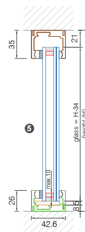
Vertical section Basis XL/ Frame XL
