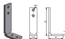
Double Glazed Frame and Top Frame or Basis Connector Cat. No. FFCCL
