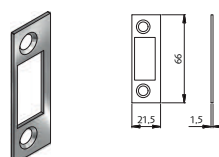
Double Glazed Striking Plate Cat. No. FXSP
