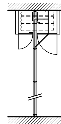
5. 'Z' system PANELS STACKED IN RECESS CUPBOARD
