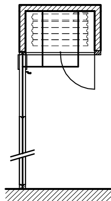
7. 'K' system PANELS STACKED IN SIDE WALL RECESS
