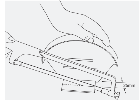
Fig. 17 – Trimming the ridge cap
