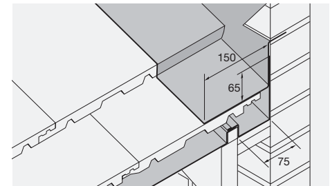
Fig. 30 – Completed secret gutter with cover flashing
