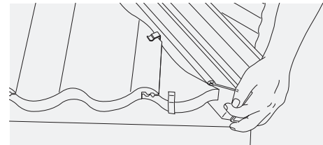
Fig. 6 – Locate hip batten section between cut tiles
