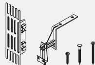
Universal dry verge starter unit (code 53931)*
