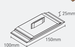
Roof Defence Intumescent Ridge Cap (code MA68010)
