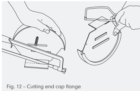
Fig. 12 – Cutting end cap flange
