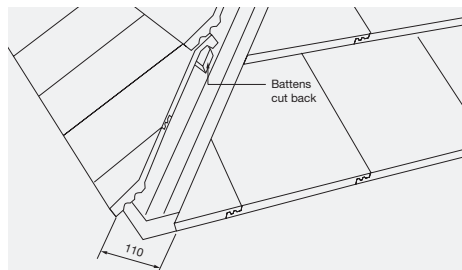
Fig. 1a – If using low profile tiles (depth less than 85mm) form a gap of 110mm at hip
