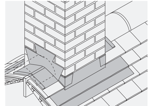
Fig. 32 – Roof chimney at ridge line
