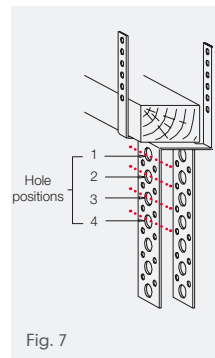
Fig. 7 Note: Bracket legs should be bent across the centres of the larger holes, as indicated by the dotted red lines.
