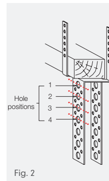
Fig. 2 Note: Bracket legs should be bent across the centres of the larger holes, as indicated by the dotted red lines.
