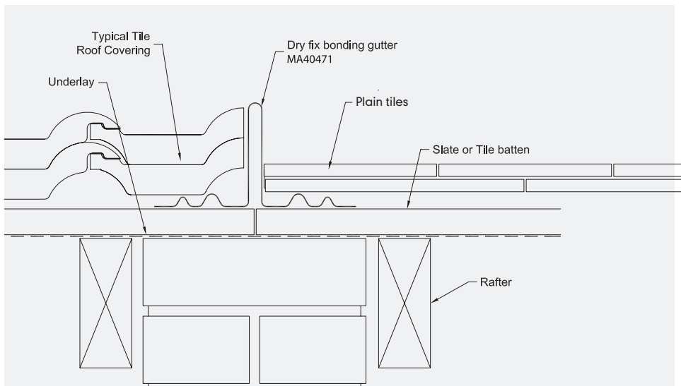
Fig. 3 – Typical standard installation showing high profiled interlocking tiles abutting slates, using 40471
