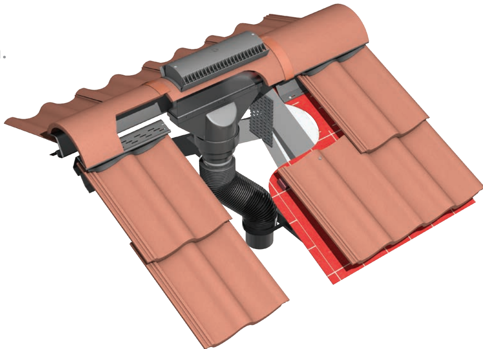
Gas vent ridge terminal for condensing boilers
