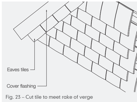
Fig. 23 – Cut tile to meet rake of verge
