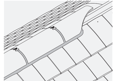
Fig. 19 – Typical bedded ridge
