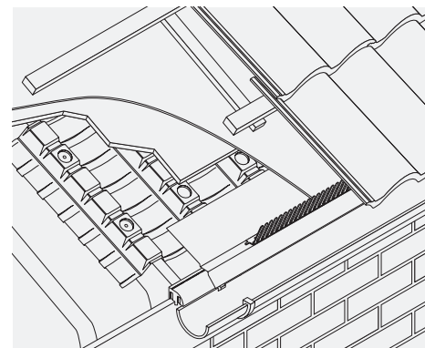
Fig. 36 – Battens and counter battens at eaves above rigid boarding and underlay
