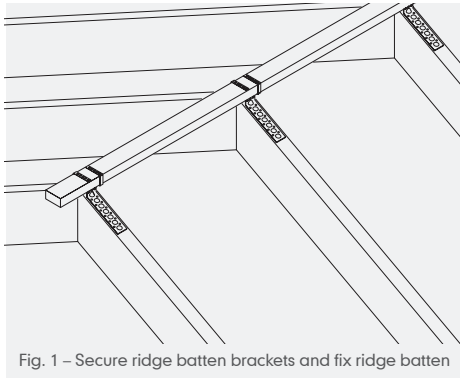
Fig. 1 – Secure ridge batten brackets and fix ridge batten
