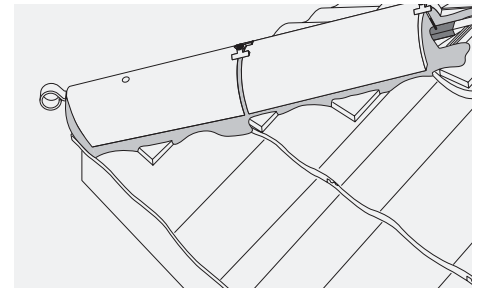
Fig. 13 – Mechanically fix hip tiles
