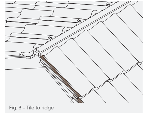
Fig. 3 – Tile to ridge
