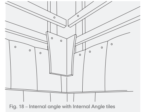
Fig. 18 – Internal angle with Internal Angle tiles
