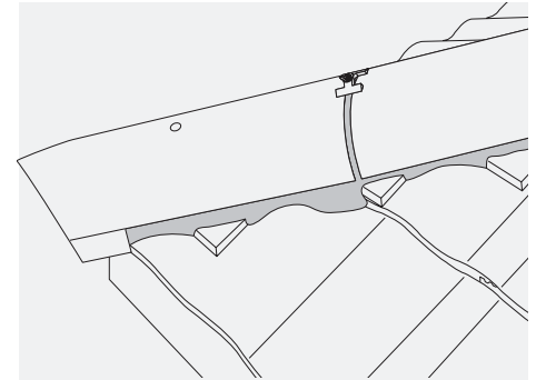
Fig. 30 – Hip end tile with mortar bedded security fixing kit
