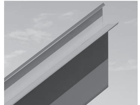
Fig. 24 – Cut trim to correct angle
