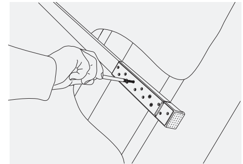
Fig. 19 – Fit extension using line moulded into unit top unit as guide
