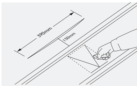
Fig. 2 – Make aperture in underlay
