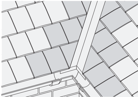
Fig. 21 – Typical bedded valley – tile-and-a-half tiles shown shaded
