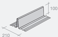
High profile bonding gutter (code 40471)
