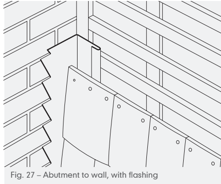
Fig. 27 – Abutment to wall, with flashing
