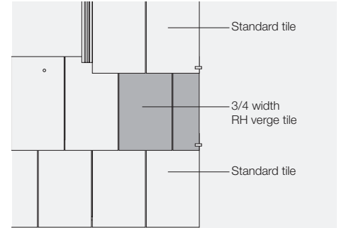
Fig. 18 – Typical bedded verge (right hand)
