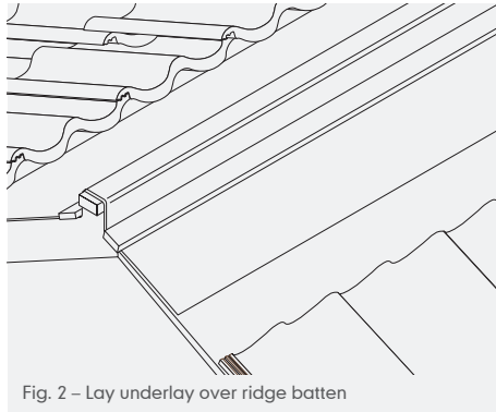
Fig. 2 – Lay underlay over ridge batten
