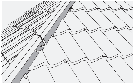
Fig. 12 – Fix hip batten
