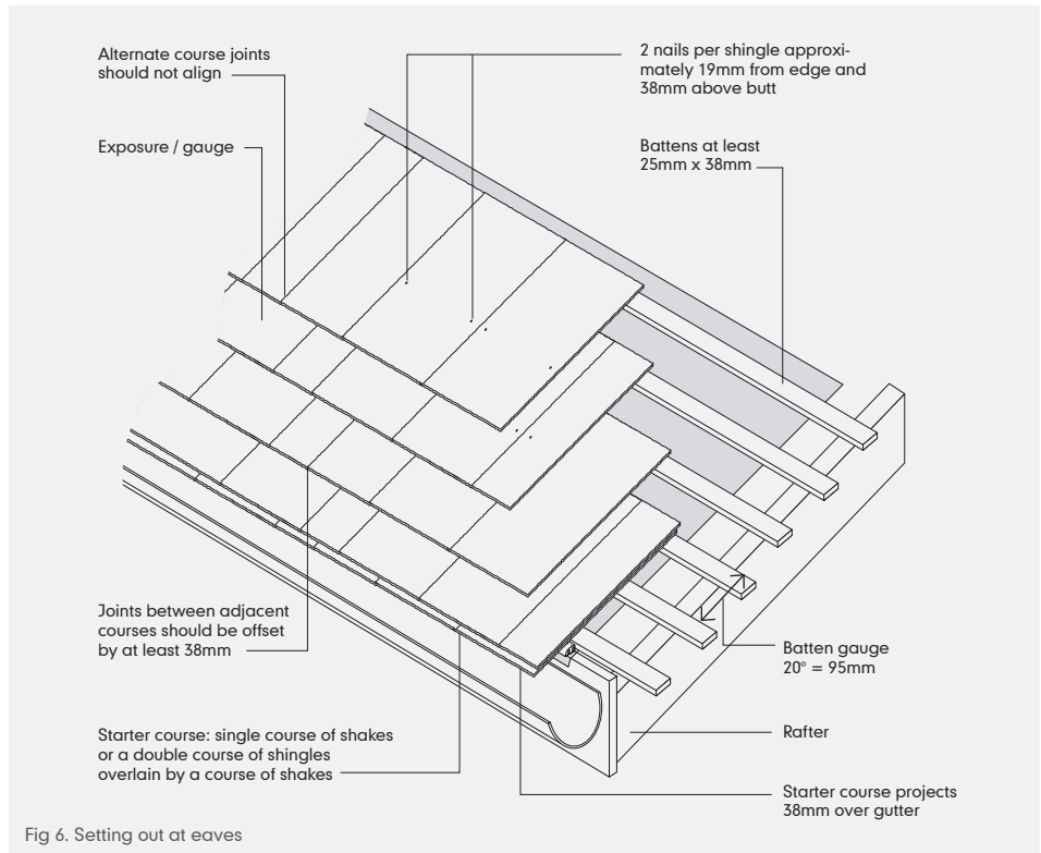
Fig 6. Setting out at eaves
