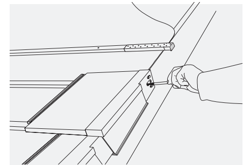
Fig. 20 – Commence installation of dry verge units in normal manner
