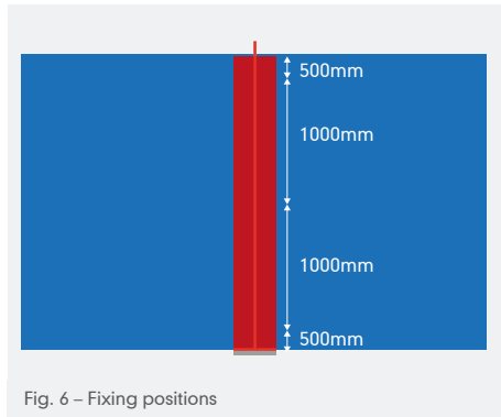
Fig. 6 – Fixing positions
