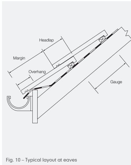
Fig. 10 – Typical layout at eaves
