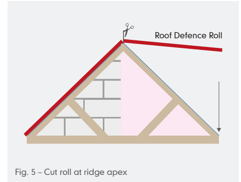
Fig. 5 – Cut roll at ridge apex
