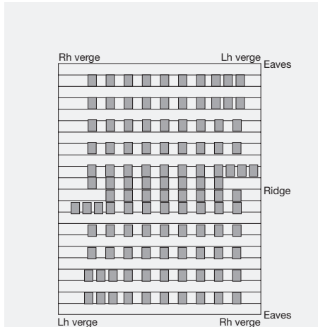
Fig. 6 – Loading roof evenly with tile/slate stacks
