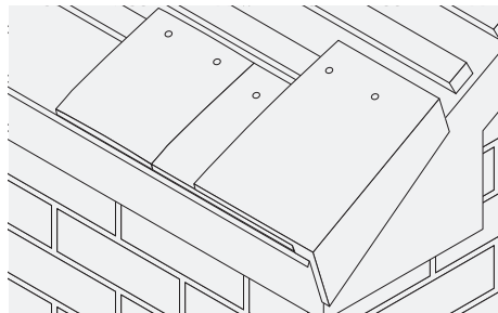
Fig. 7 - Eaves course
