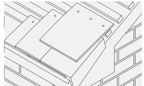
Fig. 8 - Tile-and-a-half used to break bond
