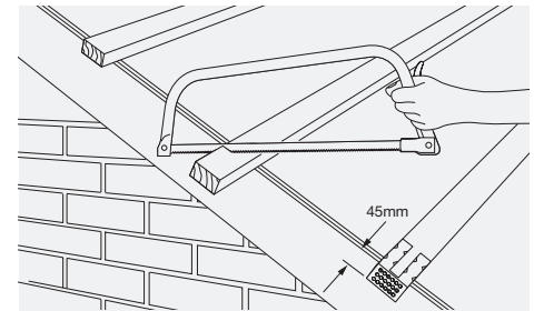
Fig. 1 – Position top course tiling battens
