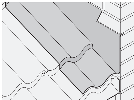
Fig. 25 – Stepped flashing with profiled interlocking tiles
