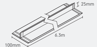
Roof Defence Intumescent Fire Barrier 6.3m (code MA68020)
