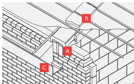
Fig. 35 – Separating wall with fire stop
