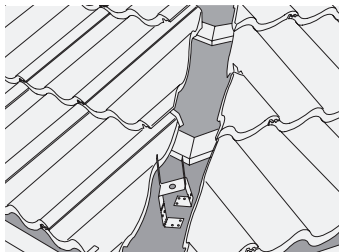
Fig. 3 - Lay tile to hip with raking cut
