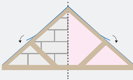
Fig. 1 – Follow plane of roof
