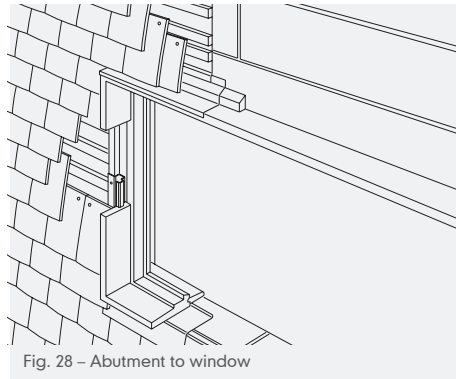
Fig. 28 – Abutment to window
