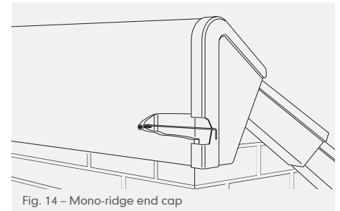
Fig. 14 – Mono-ridge end cap
