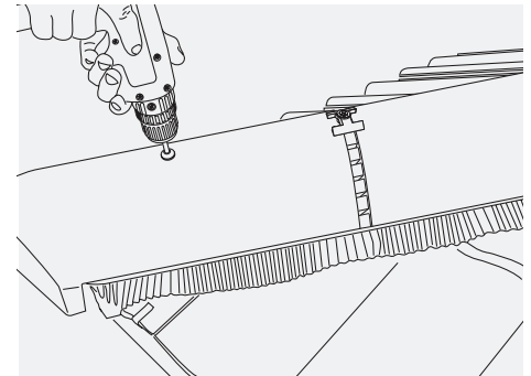
Fig. 31 – Mechanically fixed hip end using HipFast system
