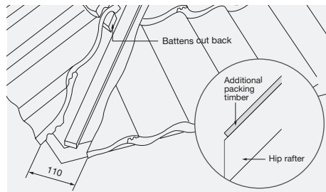
Fig. 1b – If using high profile tiles (depth more than 85mm)
