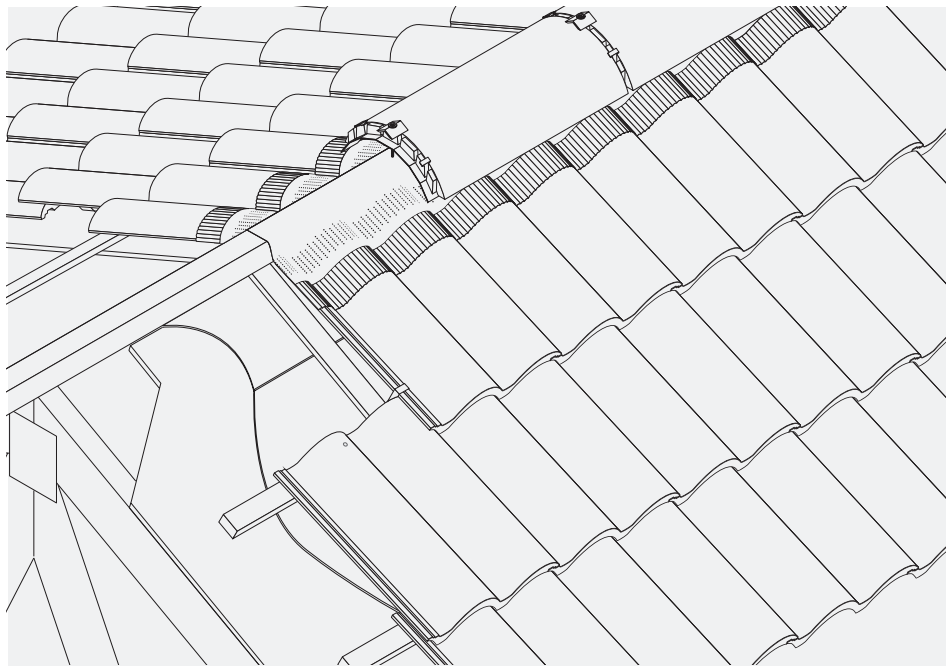
Fig. 37 – Battens and counter battens at ridge above rigid boarding and underlay (cut back at apex), with Marley ventilated dry ridge system
