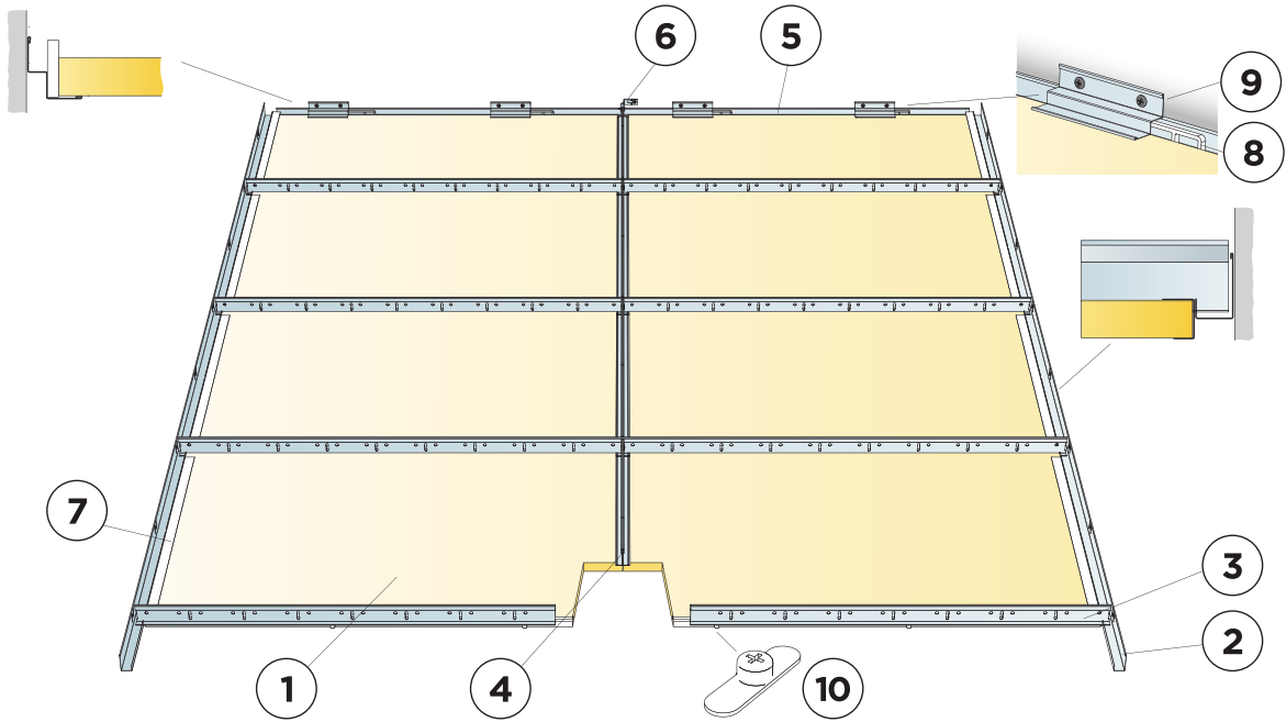
Installation diagram (M319) for Ecophon Master Rigid Dp in corridors
