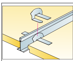
Connect Hold down clip E (patent pending)
