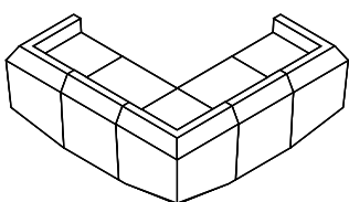
8 W2475/2475 D875 H750/900/1100 mm
