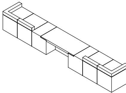
6 W6020 D875 H750/900/1100 mm
