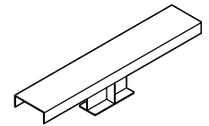
Lintel/Volume Sign-in platform Hot rolled steel W1600 × D300 × H350 mm
