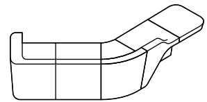
8 W3791/2159 D875 H900 mm
