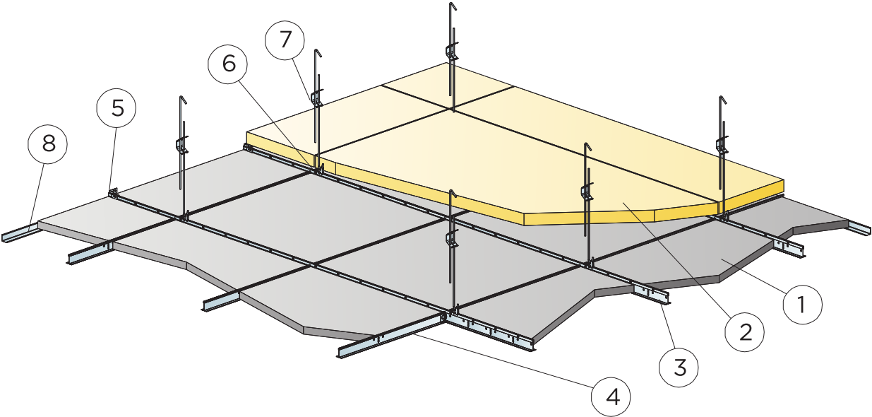
Installation diagram (M573) for Ecophon Saga A T24
