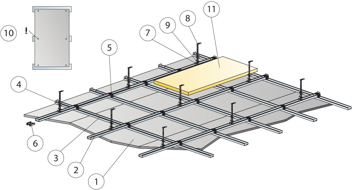
Installation diagram (M633) for Ecophon Saga B A2, suspended with grids.
