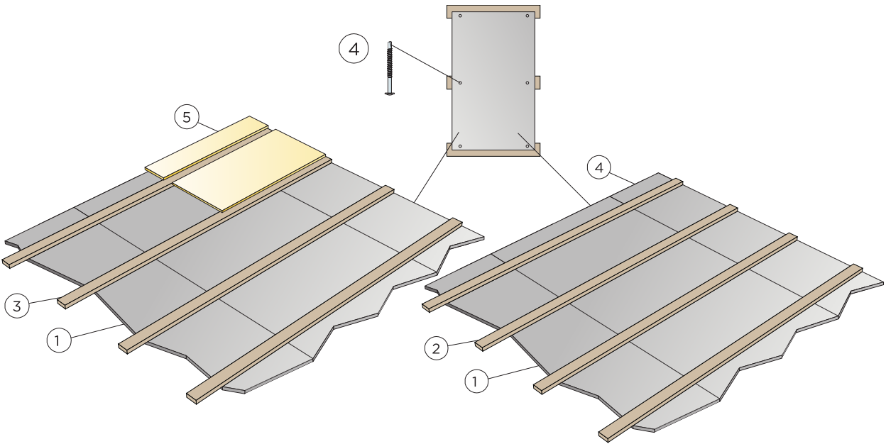
Installation diagram (M634) for Ecophon Saga B A2, direct fixing system (ceiling).
