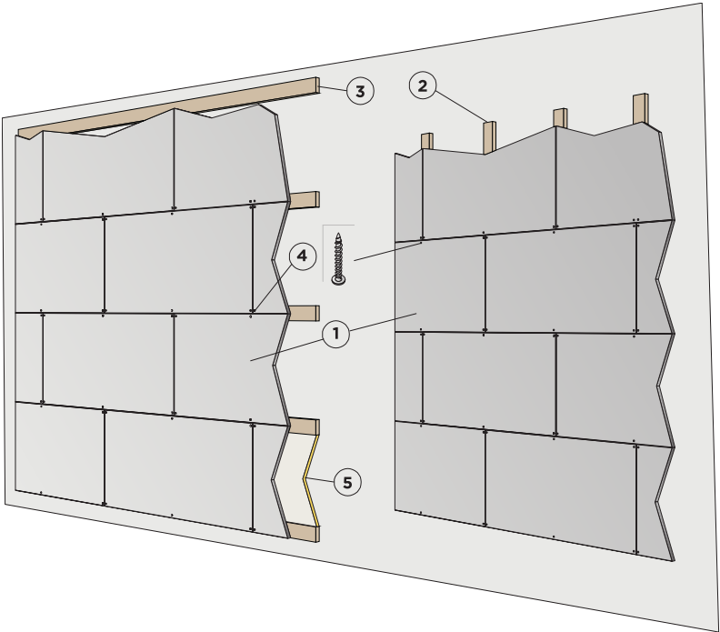
© Saint-Gobain Ecophon AB Installation diagram (M578) for Ecophon Saga B, lathing wall system.
