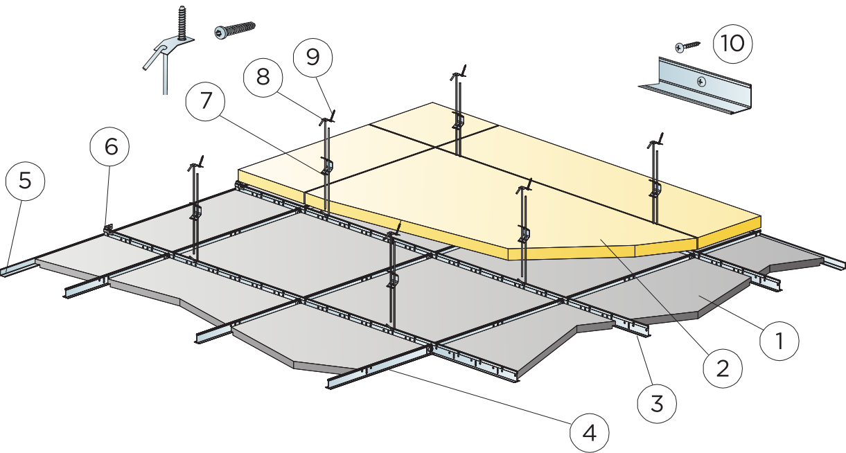
Installation diagram (M703C4) for Ecophon Saga E A2
