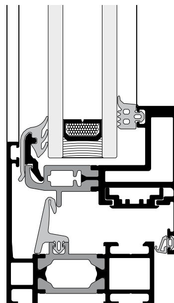
Schüco AWS 60 BS Concealed vent window with slim face widths from 67 mm
