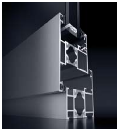
Schüco AWS 50 Outward opening window
