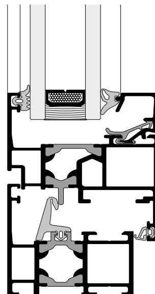
Schüco AWS 50 Thermally insulated frames with centre sealing gasket
