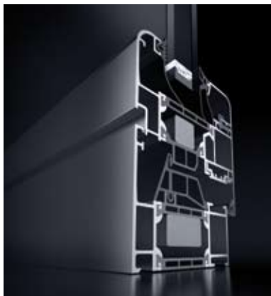
Schüco AWS 70 SL.HI Softline High Insulation window with rounded vent contour
