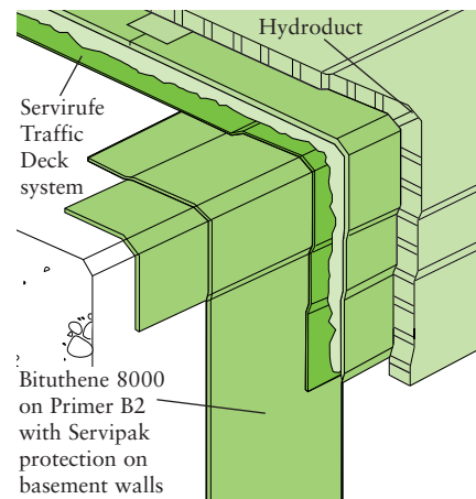
Detail of Basement Roof
