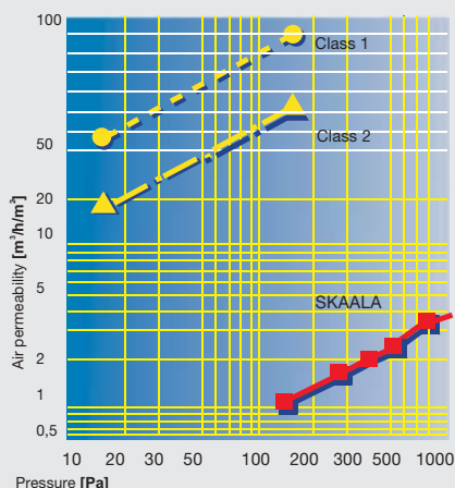
Test results, air permeability
