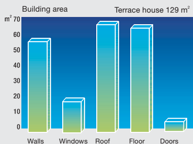
On U-Value ~1,0 W/m² the loss of energy of the windows lessens to the same level with other parts of the building.
