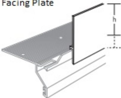
ProFin ® BL 49 Facing Plate
