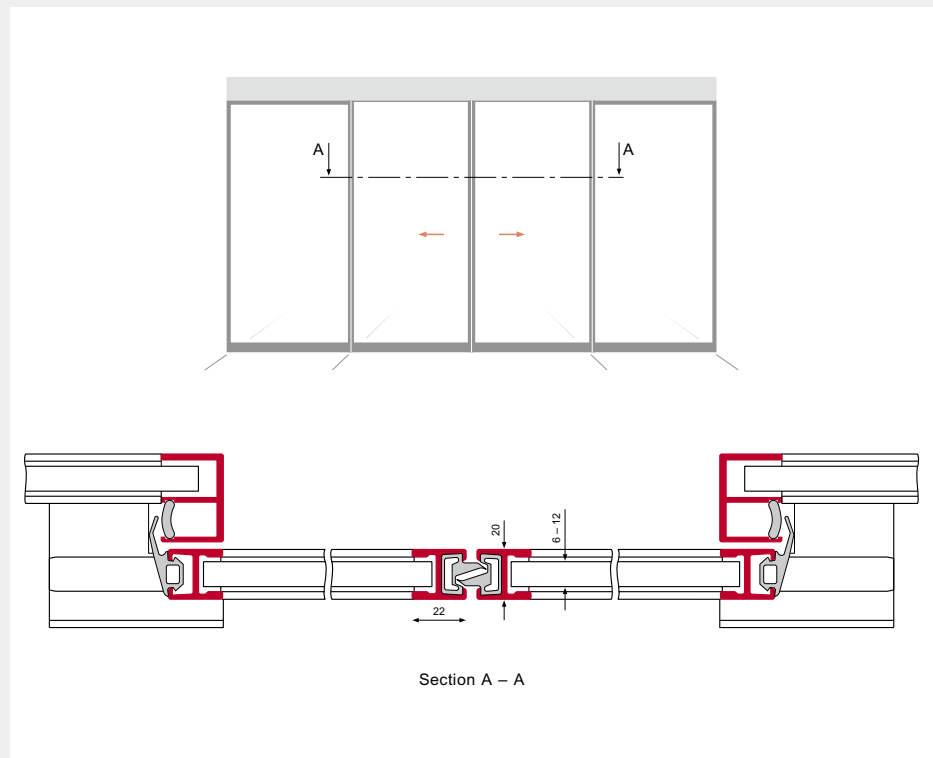
SLIDEDOOR Profile System LR 12
