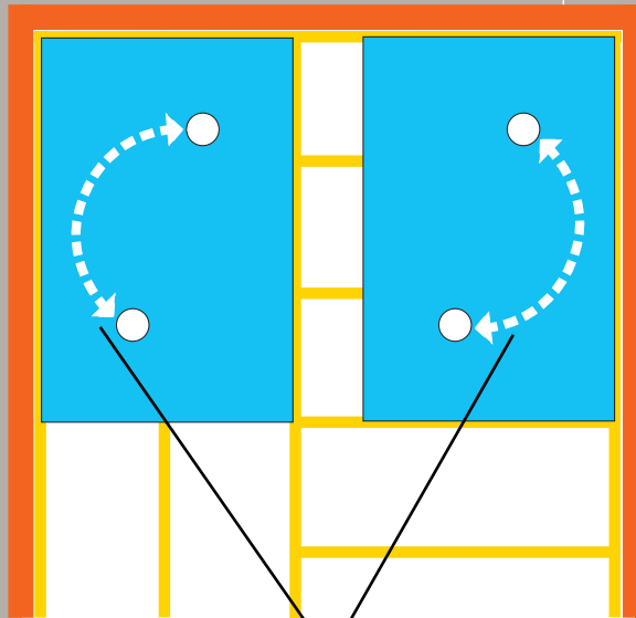
Optional drain location - rotate MAXXUS to avoid joists
