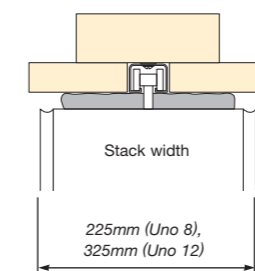
Track with acoustic seal
