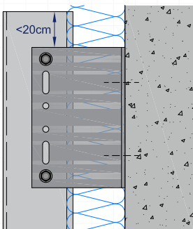
FIXED POINT
