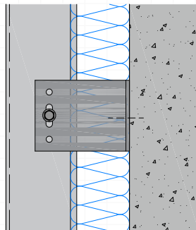
SLIDING POINT
